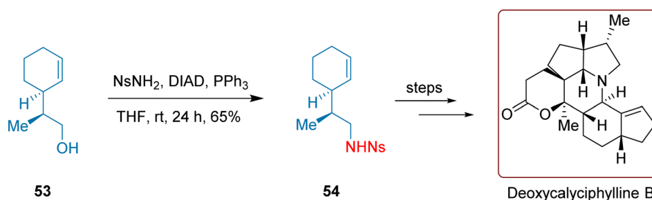
Scheme 24 Raghavan's synthesis of deoxycalciphylline B.
