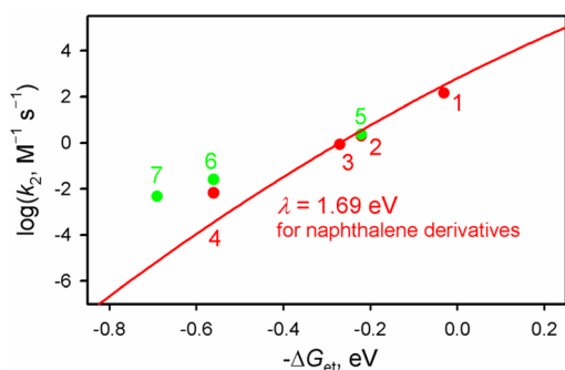
Fig. 4 Plot of \log k_2 for the oxidation of different substrates [(1) 1-Me-naphthalene, (2) naphthalene, (3) 1-Br-naphthalene, (4) 1- \text{NO}_2 -naphthalene, (5) anisole, (6) toluene, and (7) benzene] vs. the driving force of electron transfer [ -\Delta G_{\text{et}} ; eqn (2)] by 3/\text{Cl}^- in \text{CH}_2\text{Cl}_2 at -10 °C.
