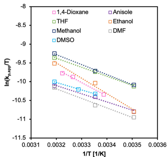
Fig. 7 Eyring–Polanyi plot for PI-RAFT synthesis of PPEGMA in various solvents. Initiated under \lambda_{\max} = 450 \text{ nm} , 18 \text{ mW cm}^{-2} , [M]_0/[I] = 100 , 50 \text{ vol\%} .
