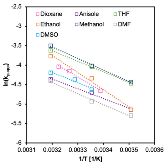
Fig. 6 Arrhenius plot for PI-RAFT synthesis of PPEGMA in various solvents. Initiated under \lambda_{\max} = 450 \text{ nm} , 18 \text{ mW cm}^{-2} , [M]_0/[I] = 100 , 50 \text{ vol\%} .
