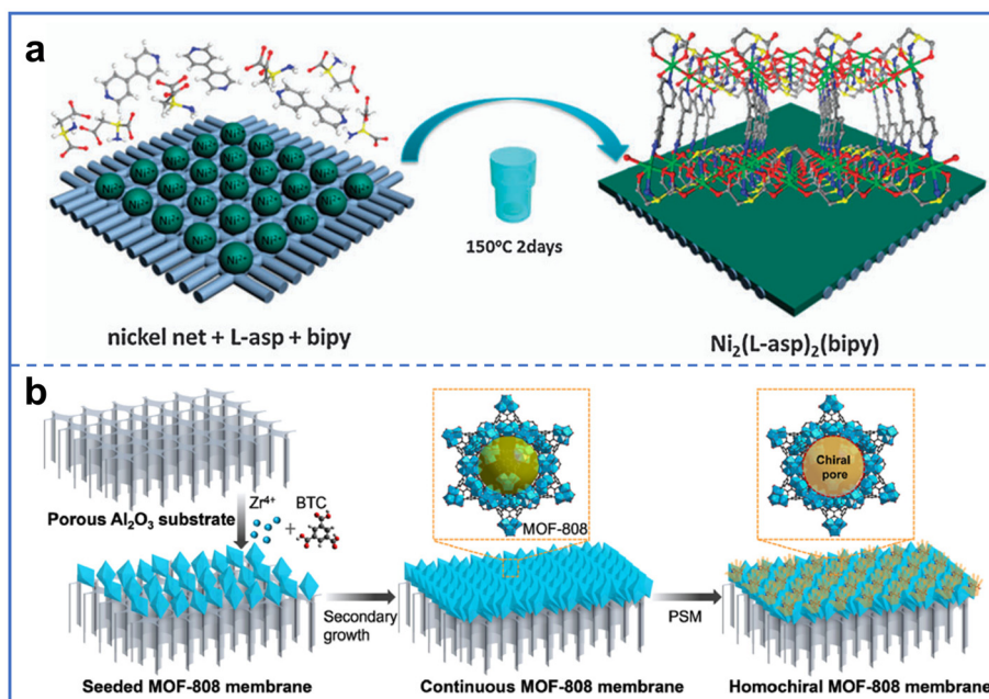
Fig. 2 (a) Preparation of thin chiral Ni 2 (L-asp) 2 (bipy) membrane with Ni net as both substrate and metal source. Reproduced with permission from ref. 27. Copyright 2013, The Royal Society of Chemistry. (b) Preparation of chiral MOF-808 membranes by introduction of chiral molecules to MOF-808 membranes. Reproduced with permission from ref. 23. Copyright 2024, American Chemical Society.
