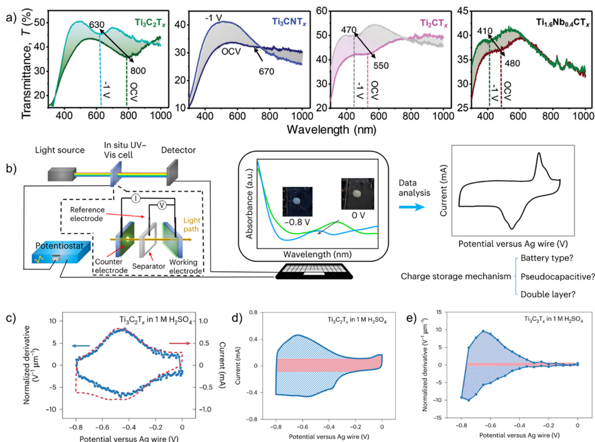
Fig. 5 (a) in situ UV-Vis spectra of Ti 3 C 2 T x , Ti 3 CNT x , Ti 2 CT x and Ti 1.6 Nb 0.4 CT x in a protic gel electrolyte comparing cathodic polarization (−1 V vs. Ag wire) with the open-circuit potential condition. 76 (b) A general workflow to determine charge storage mechanism using in situ UV-Vis spectroscopy from experimental setup to data analysis. In situ UV-Vis spectroscopy Ti 3 C 2 T x in 1 M H 2 SO 4 : (c) Electrochemical (red) and UV-Vis (blue) cyclic voltammograms (CVs), (d) electrochemical CV with the electrical double layer (EDL) contribution in red and the redox contribution in blue. Panel (a) reproduced with permission from the Royal Society of Chemistry. Panel (b–e) reproduced with permission from ref. 77, copyright 2023 Springer Nature.
