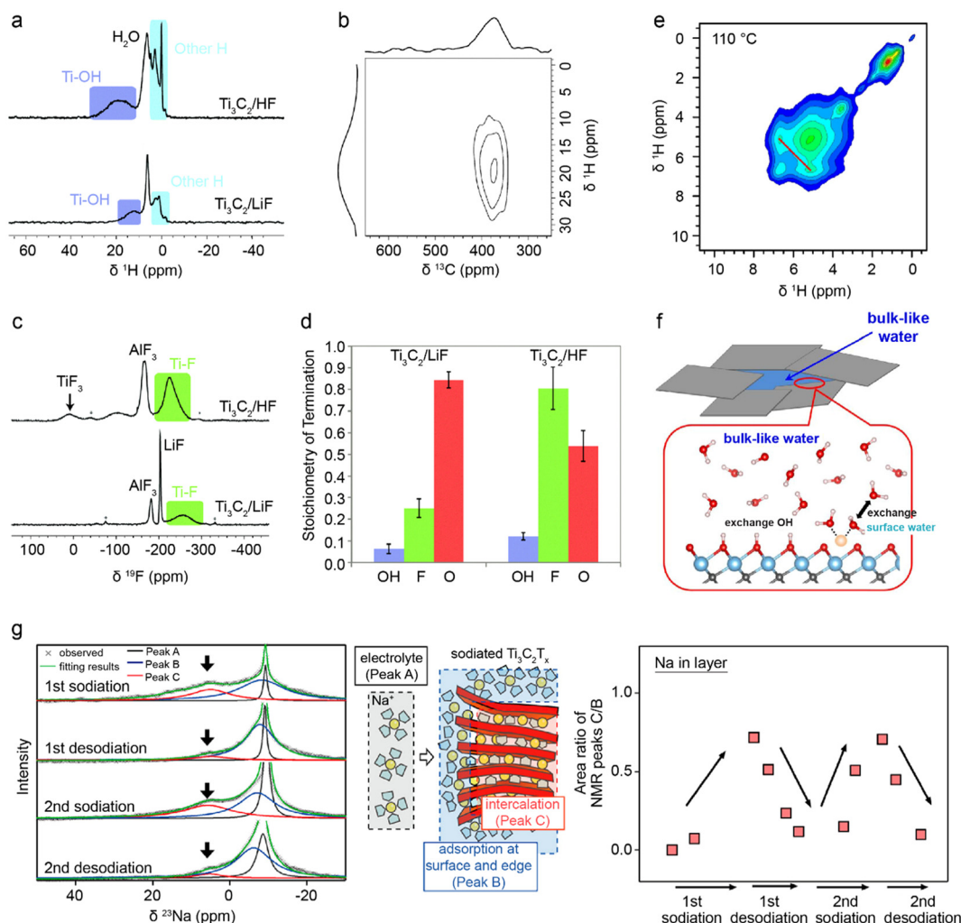
Fig. 14 MAS SSNMR study of MXene. (a) ^1\text{H} NMR spectra of HF and LiF-HCl synthesized \text{Ti}_3\text{C}_2\text{Tx} MXene recorded at 60 kHz MAS rate. 184 (b) ^1\text{H} - ^{13}\text{C} HETCOR NMR spectrum of HF synthesized \text{Ti}_3\text{C}_2\text{Tx} MXene recorded at 40 kHz MAS rate. 184 (c) ^{19}\text{F} NMR spectra of HF and LiF-HCl synthesized \text{Ti}_3\text{C}_2\text{Tx} MXene recorded at 60 kHz MAS rate. 184 (d) NMR-derived composition of the \text{Ti}_3\text{C}_2\text{Tx} surface functional groups synthesized via the HF and LiF-HCl routes. 184 (e) 2D ^1\text{H} - ^1\text{H} homonuclear correlation NMR spectrum of \text{Ti}_3\text{C}_2\text{Tx} annealed at 110^\circ\text{C} . 185 (f) Suggested model for \text{Ti}_3\text{C}_2(\text{OH})_x MXene with exchangeable water molecules between the interlayer bulk and surface. White: hydrogen, red: oxygen, orange: lithium, blue: titanium, grey: carbon. 185 (g) ^{23}\text{Na} NMR spectra of \text{Ti}_3\text{C}_2\text{Tx} after two cycles of sodiation and desodiation. The red component is assigned to the intercalated sodium, the blue component is assigned to the surface and edge sodium, and the black component is assigned to the electrolyte sodium ions. The plot on the right shows the signal integral ratio of the C to B component. 189 Panel (a–d) reproduced from ref. 184 with permission from the Royal Society of Chemistry. Panel (e and f) reproduced with permission from ref. 185, copyright 2020 American Chemical Society. Panel (g) reproduced with permission from ref. 189, copyright 2016 American Chemical Society.
