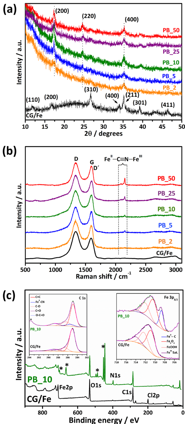
Fig. 3 X-ray diffractograms (a) and Raman spectra ( \lambda = 633\text{ nm} ) (b) of the CG/Fe (black line), PB_2 (orange line), PB_5 (blue line), PB_10 (green line), PB_25 (purple line), and PB_50 (red line) samples. XPS spectra of the CG/Fe and PB_10 samples (c).
