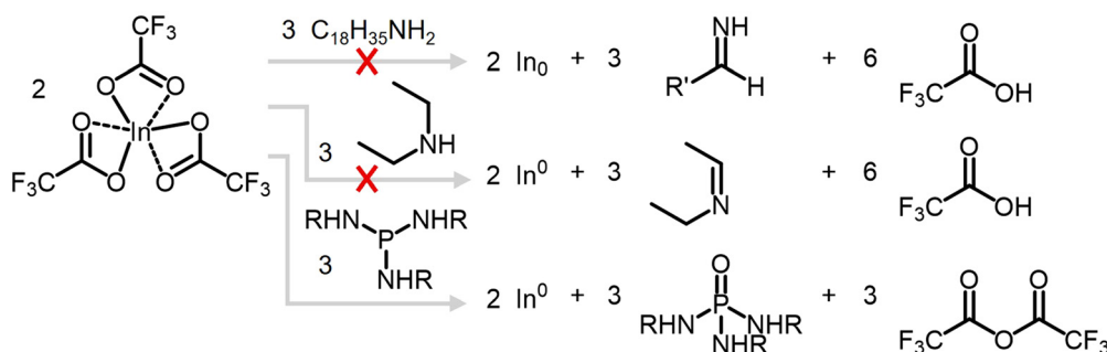
Scheme 2 Options for the reduction of indium (R = C 18 H 35 , R' = C 17 H 33 ).
