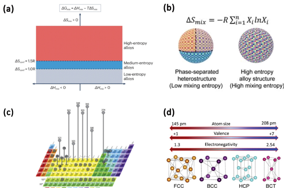
Fig. 1 (a) Basic definition of high-entropy alloys, in which \Delta G_{\text{mix}} , \Delta H_{\text{mix}} , \Delta S_{\text{mix}} and T are the Gibbs free energy of mixing, the entropy of mixing and the temperature, respectively. Reproduced from ref. 38 with permission from Nature, Copyright 2024. (b) Schematic comparison of phase-separated heterostructures synthesized by conventional slow reduction (slow kinetics) versus solid-solution HEA-NPs produced by the fast-kinetics CTS method. Reproduced from ref. 39 with permission from John Wiley and Sons, Copyright 2024. (c) The frequency of element usage in 408 multi-principal element alloys (MPEAs). Reproduced from ref. 7 with permission from Elsevier, Copyright 2017. (d) Transition metal elements and their significantly varied physicochemical properties in extreme alloying through high-temperature, high-entropy synthesis. Reproduced from ref. 40 with permission from Elsevier, Copyright 2021.
