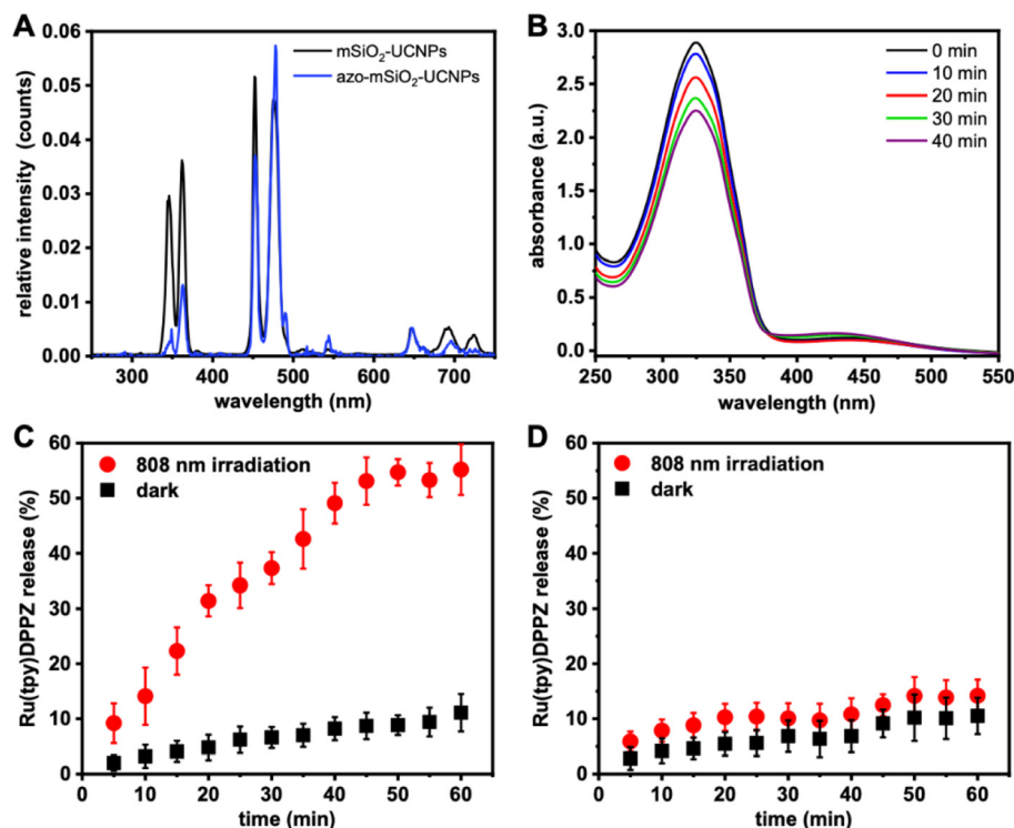
Fig. 3 (A) UCL spectra of \text{mSiO}_2 -UCNPs (black) and \text{azo-mSiO}_2 -UCNPs (blue) dispersed in \text{H}_2\text{O} upon 808 \text{ nm} NIR excitation. (B) Absorption spectra of \text{azo-mSiO}_2 -UCNPs before and after irradiation with 808 \text{ nm} NIR light for up to 40 \text{ min} . Release profiles of \text{Ru}(\text{tpy})\text{DPPZ} from \text{azo-mSiO}_2 -UCNPs (C) and \text{mSiO}_2 -UCNPs (D) with and without NIR irradiation. Standard deviations are shown as error bars for triplicate experiments.
