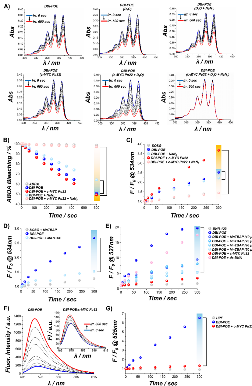
Fig. 3 (A) ABDA bleaching experiments under various conditions. Samples contained ABDA = 30 μM, NaN 3 = 10 mM, DBI-POE = 5 μM, and c -MYC Pu22 = 5 μM in 50 mM Tris (pH 6.8) with 100 mM KCl. Where indicated, D 2 O was used in place of H 2 O. (B) ABDA bleaching at 380 nm expressed as a percentage, showing that NaN 3 had negligible effects on DBI-POE alone but fully scavenged the DBI-POE : c -MYC Pu22 complex. (C) SOSG fluorescence enhancement under similar conditions: SOSG = 10 μM, NaN 3 = 10 mM, DBI-POE = 5 μM, and c -MYC Pu22 = 5 μM in 50 mM Tris (pH 6.8) with 100 mM KCl, \lambda_{\text{exc}} = 488 nm (D) SOSG fluorescence enhancement mediated by DBI-POE was quenched by MnTBAP = 50 μM. (E) DHR-123 fluorescence enhancement under varying conditions: DHR-123 = 10 μM, MnTBAP = 0–50 μM, DBI-POE = 5 μM, c -MYC Pu22 = 5 μM, and ds-DNA = 5 μM in 50 mM Tris (pH 6.8) with 100 mM KCl, \lambda_{\text{exc}} = 488 nm. In all experiments, irradiation was performed at 485 ± 20 nm at an irradiance of 10 mW cm -2 over various time intervals. (F) Fluorescence enhancement of HPF (5 μM) in the presence of DBI-POE (5 μM), or in complex with c -MYC Pu22 (5 μM) as shown in the inset. (G) Fold change in HPF fluorescence under different conditions: HPF = 5 μM, DBI-POE = 5 μM, c -MYC Pu22 = 5 μM, in 50 mM Tris (pH 6.8) with 100 mM KCl, \lambda_{\text{exc}} = 490 nm. In all experiments, irradiation was performed at 485 ± 20 nm at an irradiance of 10 mW cm -2 over various time intervals.
