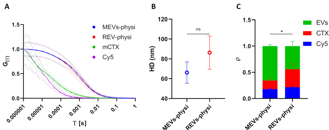
Fig. 3 (A) Normalized fluorescence correlation graphs of MEVs-physi (blue) and REVs-physi (red), mCTX (green), and Cy5 (violet). The dotted lines represent the standard deviation of the respective autocorrelation function (solid lines). (B) HD extrapolated from autocorrelation functions of physisorbed MEVs and REVs. (C) Fractions of fluorescent components in each preparation. \rho indicates the fraction of each component, namely Cy5 (blue), mCTX (red), and EVs (green).
