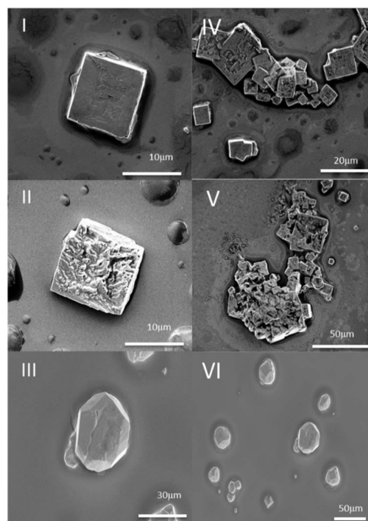
Fig. 2 HR-SEM images of \text{KIO}_3 crystals – control (I, IV/10, 20 μm), L-Arg-induced \text{KIO}_3 (II, V/10, 50 μm) and D-Arg-induced \text{KIO}_3 (III, VI/30, 50 μm).
