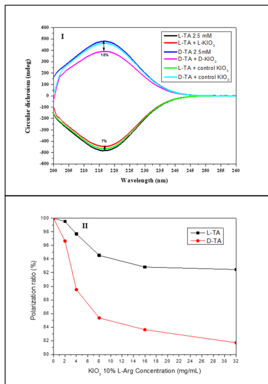
Fig. 6 Selective chiral adsorption of TA on chiral L-Arg-induced \text{KIO}_3 crystals: CD spectra of L/D-TA adsorbed onto L-Arg-induced \text{KIO}_3 (I) and selectivity of L/D-TA at different concentrations (II).
