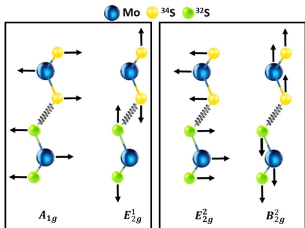
Fig. 2 In-plane, out-of-plane ( A_{1g} and E_{12g}^1 ) and inter-layer ( E_{2g}^2 and B_{2g}^2 ) phonon modes of the IHS of \text{MoS}_2(^{32}\text{S})/\text{MoS}_2(^{34}\text{S}) .
