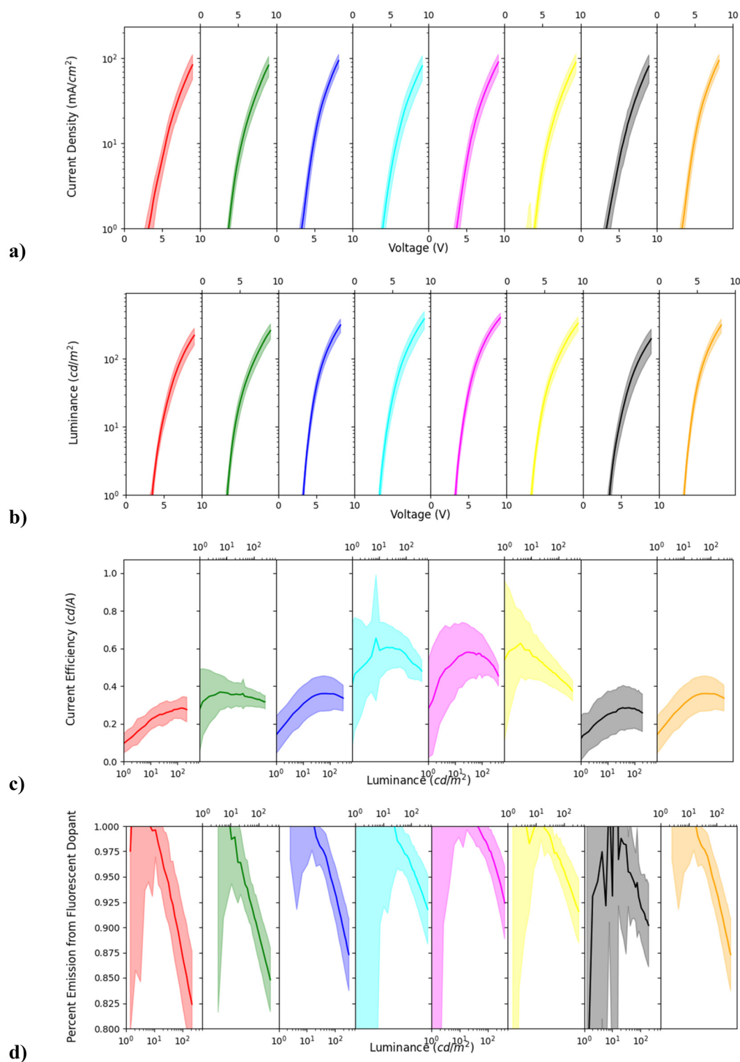
Fig. 4 Average optoelectronic properties for each set of baseline OLEDs from BsubPc material 1 (left) to material 8 (right) ( 1–8 being the axial substituents, Fig. 1). The properties shown are (a) current density as a function of applied voltage, (b) measured luminance output as a function of applied voltage, (c) current efficiency as a function of luminance output and (d) estimated contribution from the fluorescent dopant as a function of luminance output, estimated by separating the blue and orange emission components as illustrated in Fig. 7. The shaded area represents the standard deviation within the set of compositionally variant devices.
