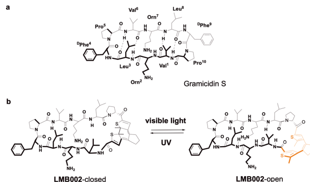
Fig. 1 Prototype of peptide GS (a) and its photoisomerizable analogue LMB002 in two photostates (b). Photoisomerizable diarylethene fragment is highlighted in peach (“open” photoisomer) or grey (“closed” photoisomer) colours.
