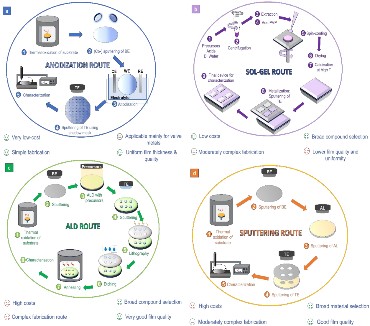
Figure 2: Typical fabrication steps of the AL by (a) anodization 31 (b) sol-gel 32 (c) ALD 101 (d) sputtering 102 routes
