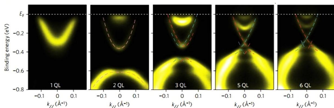
Fig. 8 Experimental ARPES spectra of few quintuple layers of bismuth selenide from ref 42 . Reprinted with permission from ref 42 .
