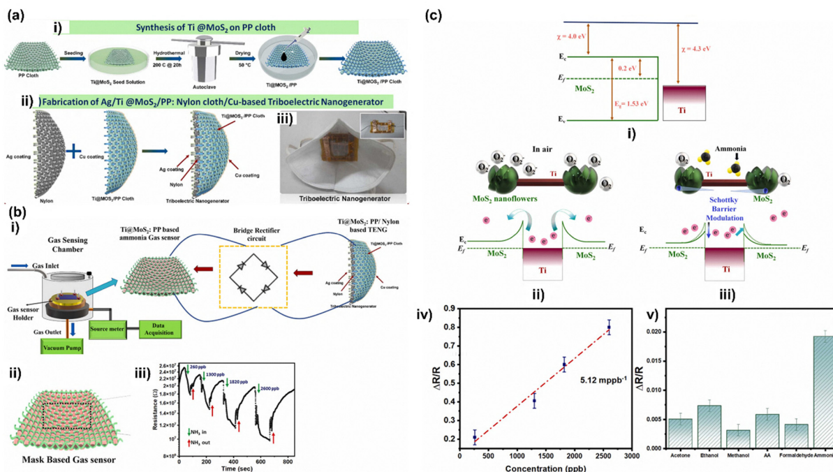
Fig. 8 (a) (i) Synthesis of \text{Ti@MoS}_2 on PP Cloth, (ii) steps for the fabrication of the \text{Ag/Ti@MoS}_2/\text{PP/Nylon/Cu} triboelectric nanogenerator, and (iii) real-time representation of the triboelectric mask nanogenerator. (b) (i) Schematic of the gas sensing chamber and the integrated self-powered ammonia gas sensing setup, (ii) schematic displaying the structure of the mask-based gas sensor, and (iii) the dynamic gas sensing response towards an increase in the concentration of ammonia. (c) (i) Band diagram of the \text{Ti@MoS}_2 structure; charge transport mechanism and band diagram of the \text{Ti@MoS}_2 gas sensor in an (ii) air atmosphere and (iii) ammonia atmosphere; (iv) calibration plot of the gas sensor displaying a sensitivity of 0.512 \text{ ppb}^{-1} , and (v) selectivity studies towards co-existing species. (Reprinted with permission, 49 Copyright 2023, Elsevier.)
