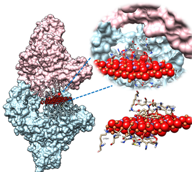
Fig. 14 Molecular docking results of quercetin (grey spheres) in the BSA–MnFe 2 O 4 (101) complex. The BSA protein surface in light blue (chain A) at the bottom and pink (chain B) at the top. The (101) facet (red/copper spheres, van der Waals representation) and key interacting amino acid residues are labeled.
