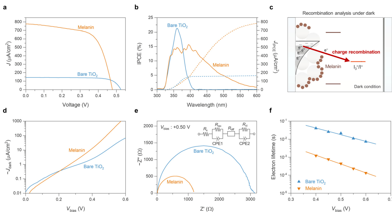
Fig. 3 Comparing the melanin-DSSC and the unsensitized bare-TiO 2 DSSC with charge recombination analysis in dark conditions. (a) J - V curves obtained under standard AM 1.5G sunlight at 100 mW cm -2 , employing a mask to prevent the issue of overestimation. (b) IPCE spectra (solid lines) measured in DC mode, along with the integrated photocurrent calculated from these IPCE spectra ( J IPCE , dotted lines). (c) Schematic representation of characterizing melanin-DSSCs in dark conditions, demonstrating the occurrence of charge recombination between TiO 2 and the electrolyte without any photoinduced charge transfer process. (d) Dark current curves of the DSSCs. (e) and (f) EIS analyses of the DSSCs: (e) features Nyquist plots with a corresponding equivalent circuit model obtained at a +0.50 V bias under dark conditions, and (f) shows the variations in electron lifetime as a function of V bias ranging from +0.40 V to +0.60 V. The electron lifetime is determined using the equation \tau = 1/(2\pi f_p) , where f p represents the peak frequency found in the mid-frequency region of the Bode phase plots (refer to Fig. S3, ESI†).
