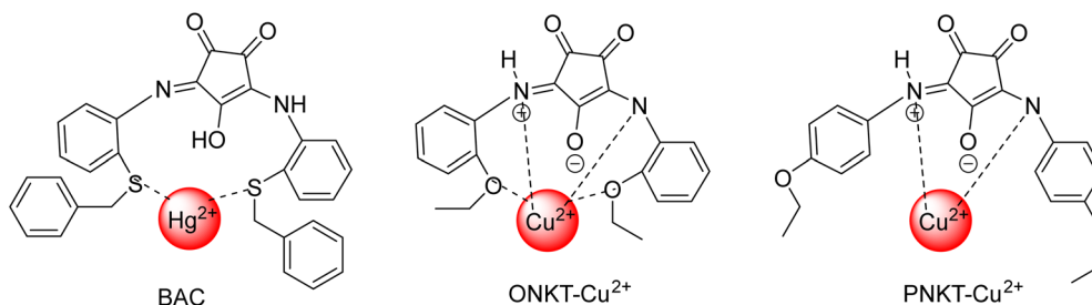
Fig. 18 CRs: BAC binding Hg^{2+} and ONKT and PNKT binding Cu^{2+} .
