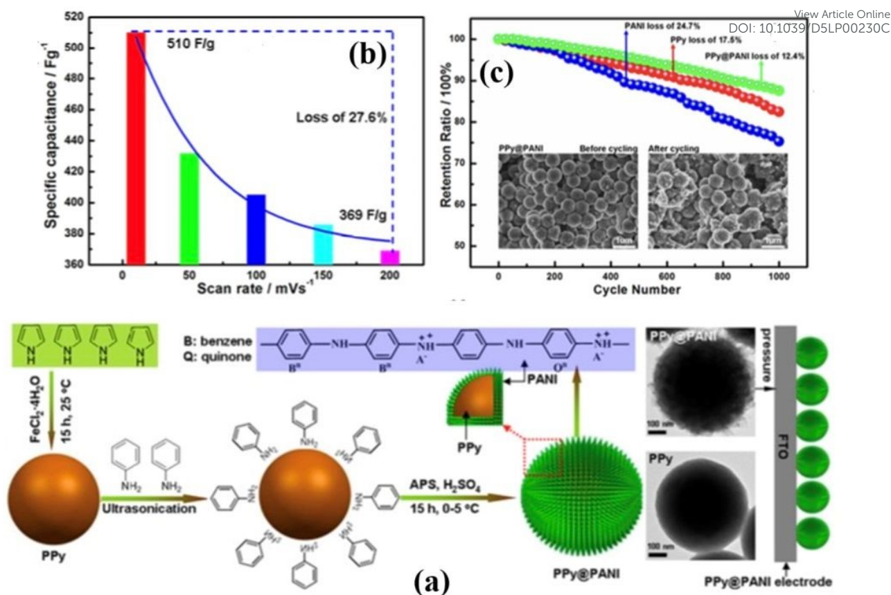
Figure 38 (a) Schematic diagram for the synthesis of core-shell PPy@PANI nanospheres. (b) SC values' plot of the scan rates and (c) Charge/discharge cycling of the core-shell PPy@PANI-0.008, individual PPy, and the PANI electrode are carried out at 5 A/g in \text{H}_2\text{SO}_4 aqueous electrolyte (1 M). The insert is the SEM images of the core-shell@PANI-0.008 before and after 1000 cycles. 585 Reproduced with permission from ACS.
