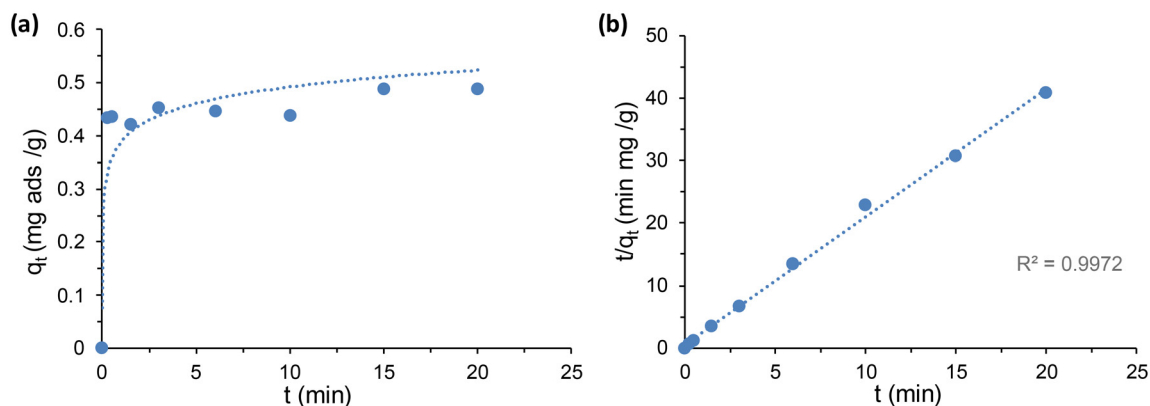
Fig. 6 (a) Hg(II) adsorption kinetics of Zr-MSA-UV2 for 20 minutes contact. (b) The pseudo-second-order kinetic plot for the adsorption (Hg(II) concentration of 10 \text{ mg L}^{-1} ).
