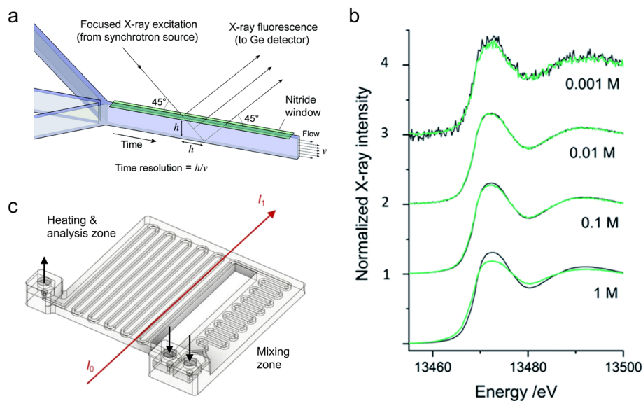
Fig. 6 Devices for hard XAS analysis. (a) Design of a microfluidic device with a silicon nitride window for XAS in fluorescence mode (adapted with permission from Chan et al. , 2007; Copyright 2007 American Chemical Society). 156 (b) Br K-edge XANES spectra of aqueous NaBr solutions at the indicated molar concentrations. The dark grey curves are from transmission detection and the green curves are from fluorescence detection (adapted with permission from Micheal Raj et al. , 2021; Royal Society of Chemistry). 159 (c) Design of a 3D-printed millifluidic device for XAS in transmission mode (adapted with permission from Dobrovolskaya et al. , 2023; Copyright 2023 American Chemical Society). 166
