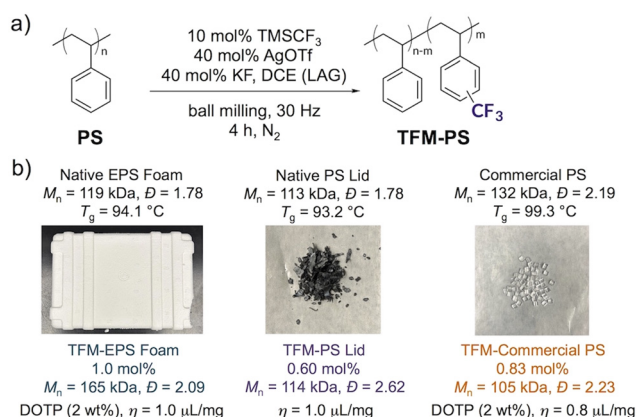
Fig. 14 (a) Electrophilic trifluoromethylation strategy for grafting polystyrene by ball milling. (b) Examples of post-consumer and commercial polystyrene samples functionalized with CF 3 groups under LAG conditions and in the presence of DOTP plasticizer. Adapted with permission from M. E. Skala, S. M. Zeitler and M. R. Golder, Liquid-assisted grinding enables a direct mechanochemical functionalization of polystyrene waste, Chem. Sci. , 2024, 15 , 10900–10907. 78
