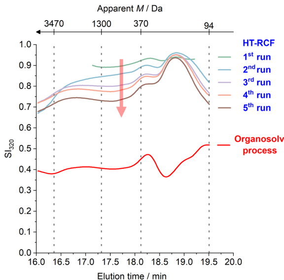
Fig. 8 SI_{320}(M) profiles of HT-RCF lignin oils from post-consumer cardboard obtained over five consecutive HT-RCF runs with RANEY ® Ni (2-propanol/ H_2O , 7 : 3 v/v; 200 °C; 3 h; H_2 -free), compared with the SI_{320}(M) profile of organosolv lignin.
