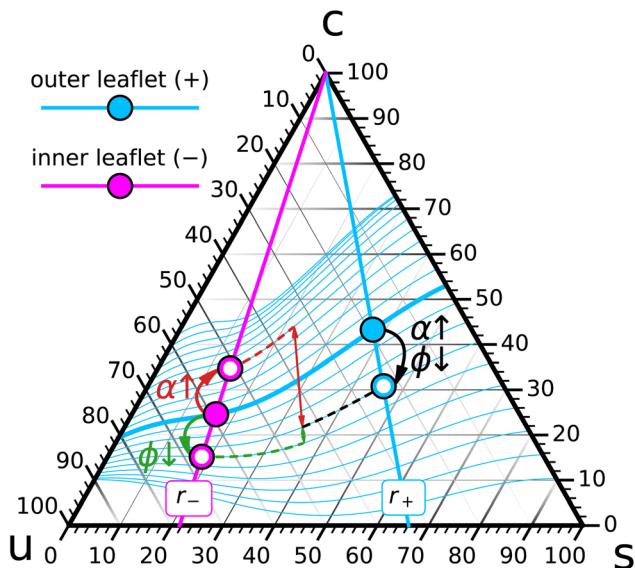
Fig. 5 Perturbation of a ternary asymmetric GUV initially set up such that its inner composition \{r_{-}, \phi_{-}\} (big magenta dot) and outer composition \{r_{+}, \phi_{+}\} (big cyan dot) chemically coexist at \mathcal{F} = 0 . The two independent perturbations which either decrease \phi or increase \alpha will have a similar effect on \text{leaf}_{+} : a reduction of \phi_{+} . But their effects on \text{leaf}_{-} are opposite: depleting cholesterol will reduce \phi_{-} while increasing \alpha will increase \phi_{-} . The extent to which this moves points that originally shared the same zero-torque foliation onto different foliation curves is very different.
