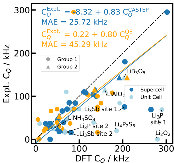
Fig. 4 Reference scale for {}^7\text{Li}\text{CQ} . The {}^7\text{Li}\text{CQ} values for 23 Li-containing compounds are calculated with PBE, fixed cell geometries, using CASTEP for unit cells (light blue), 2 \times 2 \times 2 supercells (blue), and Quantum ESPRESSO (orange) with the default PP in each case. The experimental values from literature can be found in ESI Table S4.† The dashed diagonal line indicates the limit of ideal correlation. Outliers including \text{Li}_3\text{P} and \text{Li}_3\text{Sb} are labelled and described further in the text. The data point for \text{Li}_3\text{N} [site 1] ( \text{CQ} = 582\text{ kHz} , ESI Table S4†) is beyond the depicted range, but is included in the regression analysis.
