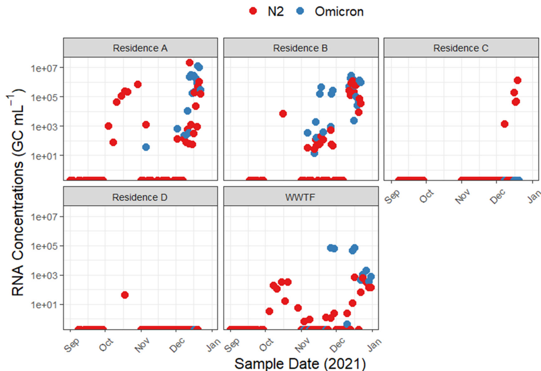
Fig. 2 Time series of SARS-CoV-2 N2 (red) and Omicron C28311T (blue) gene copies in wastewater from September 2021 to January 2022. Passive samples from four university residences and composite samples from a WWTF are displayed. Sampling dates are shown on the x-axis, while the y-axis presents the average concentration in GC mL -1 .
