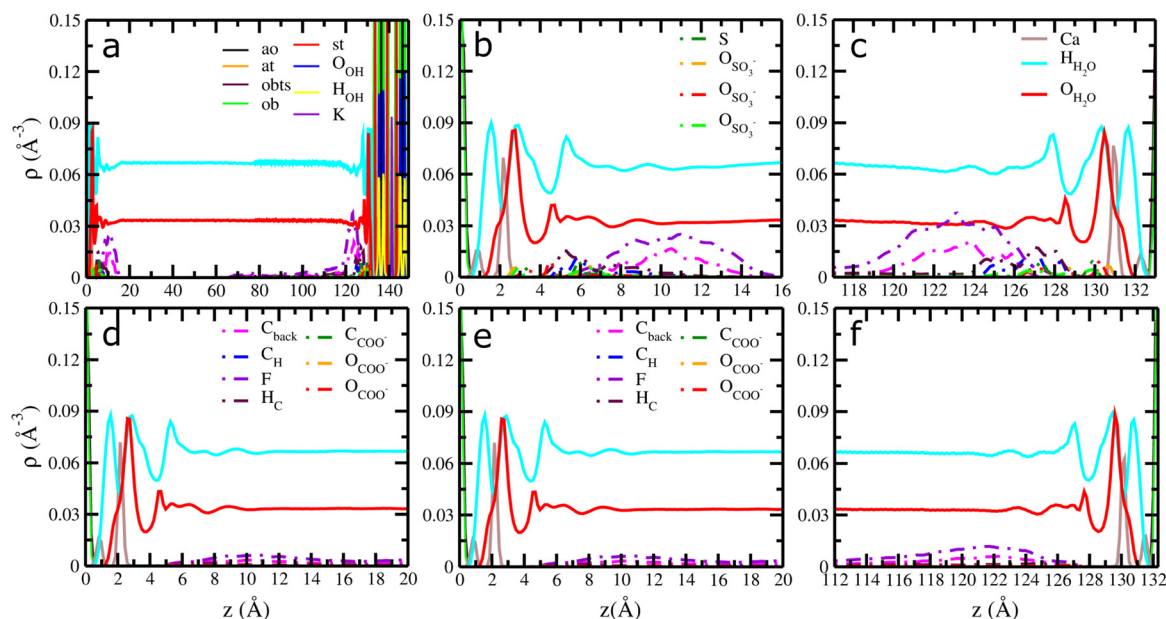
Fig. 3 Computed atomic density profiles (ADPs) of 6:2 FTS and 6:2 FTC and H 2 O molecules as a function of the distance normal to the basal surface of illite. (a–c) 6:2 FTS (d–f) 6:2 FTC. The O H2O and H 2 O are shown as solid red and cyan. Dashed lines represent the atoms of 6:2 FTS/6:2 FTC molecules. The O SO3 and S SO3 represent oxygen and sulfur atoms in 6:2 FTS and the O COO and C COO represent oxygen and carboxyl carbon atoms in 6:2 FTS. The C back , F and H c corresponds to carbon backbone, fluorine and hydrogen in each FT's. Labels – ao, at, st, ob, and obts represent surface atoms in montmorillonite following the notation used in clayff. 55 The origin ( z = 0 ) is the mean position of the basal surface 'O' atoms of illite.
