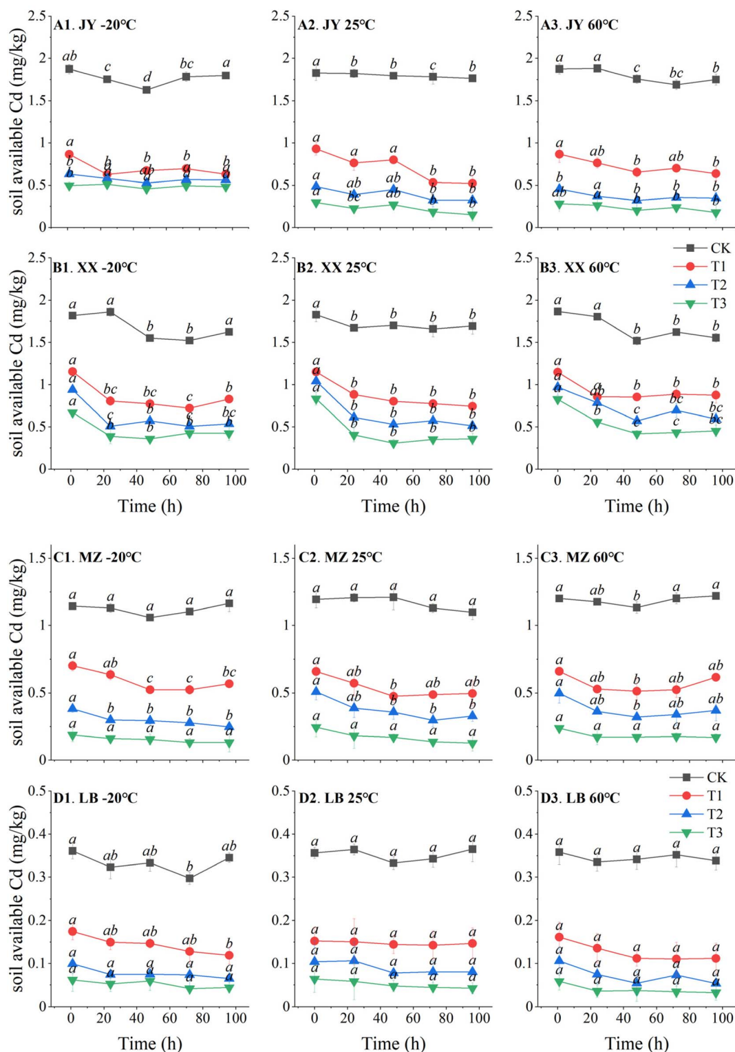
Fig. 6 Available Cd dynamics in SGP amended soils under different temperatures ((A–D): Jiyuan, Xixiang, Mianzhu, Libo soils; 1–3: –20 °C, 25 °C, 60 °C). The different lowercase letters above the data point indicate statistical differences between different sampling times for the same treatment.
