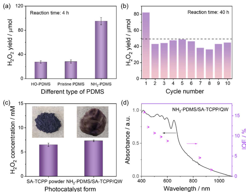
Fig. 6 (a) Comparison of the H_2O_2 yields for pristine PDMS/SA-TCPP/QW, HO-PDMS/SA-TCPP/QW, and NH_2 -PDMS/SA-TCPP/QW composites. (b) Cycling stability of the NH_2 -PDMS/SA-TCPP/QW composite over ten successive runs. (c) Comparison of the H_2O_2 yields between SA-TCPP powder and NH_2 -PDMS/SA-TCPP/QW composite at 80 °C. (Insets) Photographs showing the SA-TCPP powder (left) and the immobilized NH_2 -PDMS/SA-TCPP/QW composite (right). (d) UV-Vis-NIR absorption spectrum (black line, left axis) and incident quantum efficiency (IQE, magenta triangles, right axis) of NH_2 -PDMS/SA-TCPP/QW composite under irradiation with different monochromatic wavelengths. Solution: 30 mL H_2O , pH = 7, temperature: 40 °C, SA-TCPP catalyst loading: 45 mg, O_2 bubbling, reaction time: 4 h, light source: Xe lamp with a 420 nm cut-off filter.
