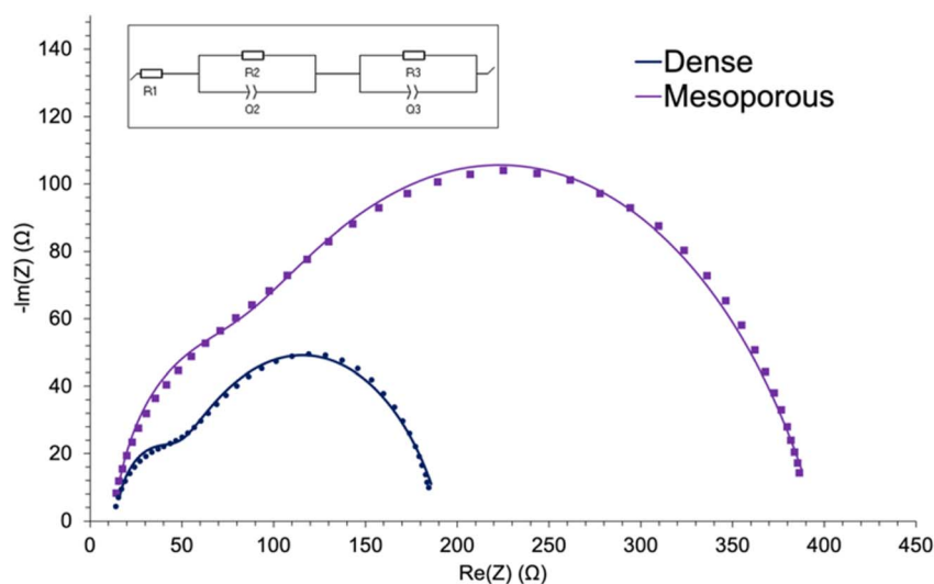
Fig. 14 EIS Nyquist plots of glass/FTO/c-TiO 2 /Sb 2 S 3 / Spiro/Au (dark blue) and glass/FTO/c-TiO 2 /mp-TiO 2 /Sb 2 S 3 / Spiro/Au (purple) solar cells; inset: the equivalent electrical circuit used for data fitting.
