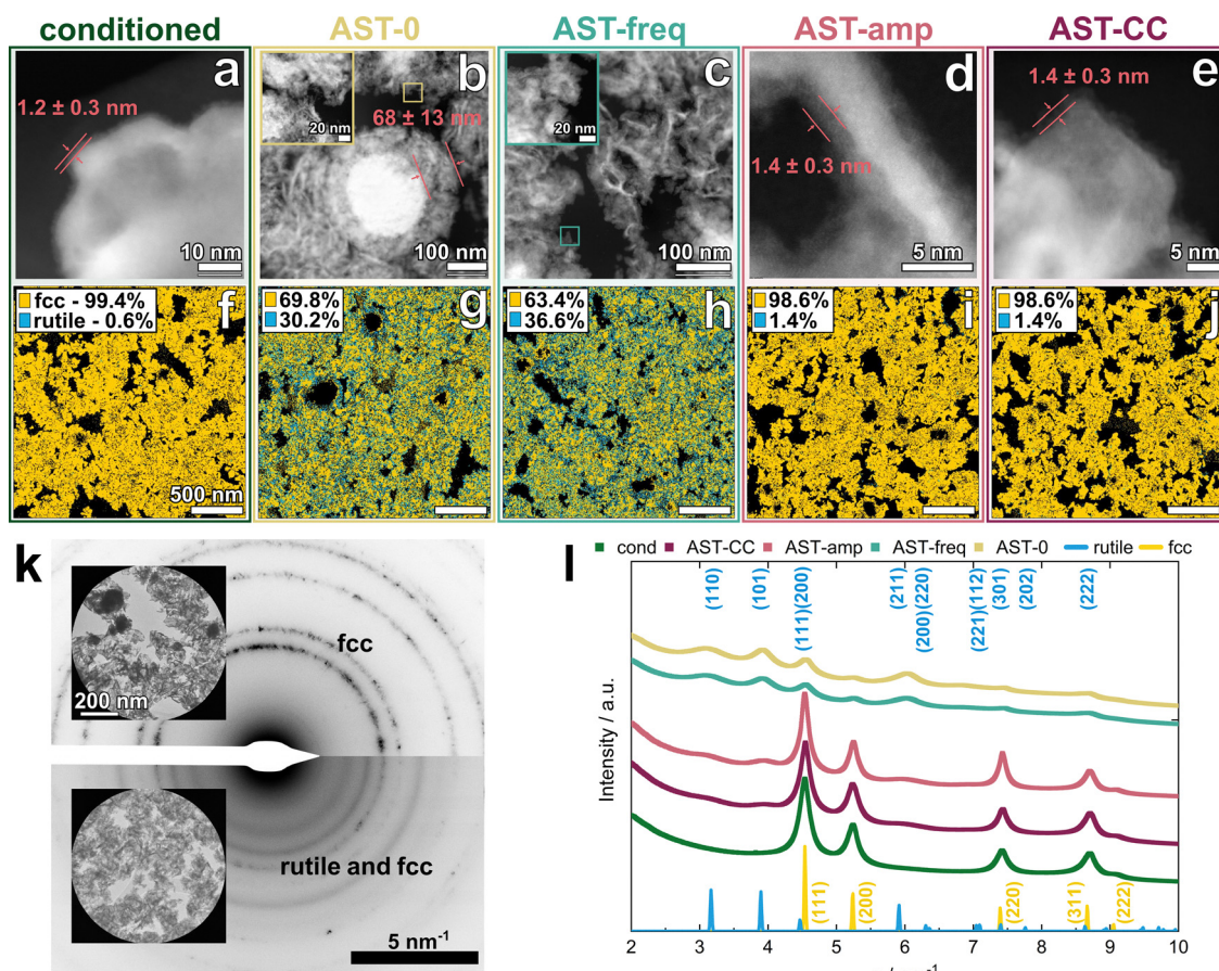
Fig. 4 Ex situ characterization of the anode catalyst layer at EOT after all stress tests and after conditioning as reference. The measurements are performed on ~100 nm slices cut with an ultramicrotome from embedded CCMs: (a)–(e) HAADF-STEM images of Ir particles within the CL. Thickness measurement of oxide thickness was performed using ImageJ. The mean value \pm standard deviation from seven points is shown. (f)–(j) Phase map from 4D-STEM showing the distribution of fcc metallic and oxidic Ir and their atomic fractions. Corresponding Bragg vector maps are shown in Fig. S14b–f. (k) Exemplary SAED pattern of CLs and corresponding selected areas as insets. Top: SAED from conditioned sample showing characteristic pattern of fcc Ir. Bottom: SAED from AST-0 showing characteristic pattern of mixed rutile IrO 2 and fcc. SAED from all stress tests can be found in Fig. S12. (l) Intensity vs. reciprocal lattice vector q of distortion-corrected SAED patterns. 52 q is the reciprocal scattering vector where 1/q corresponds to lattice plane distances in real space. Reference spectra for Ir and IrO 2 are retrieved from inorganic crystal structure database (ICSD). Note that the plots are intensity normalized and shifted along the y -axis to improve readability. See Fig. S14a for raw data.
