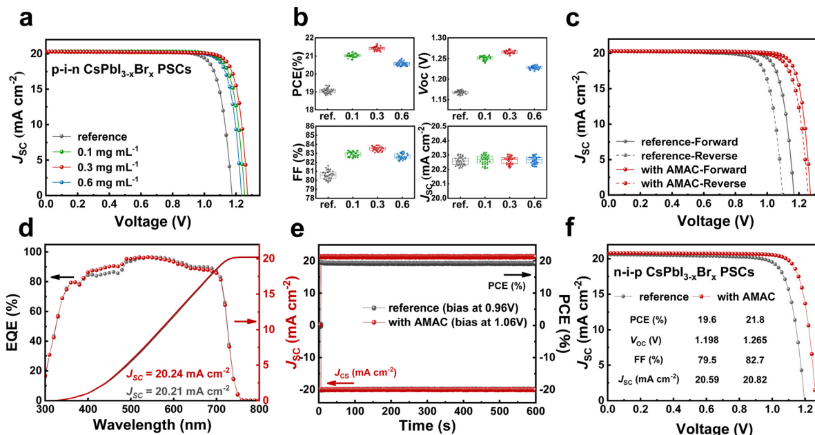
Fig. 4 (a) J - V characterization of p-i-n CsPbI 3-x Br x PSCs incorporated with different amounts of AMAC under 100 mW cm -2 illumination (the active area is 0.09 cm 2 ). (b) Statistical box charts of PV parameters. (c) Hysteresis with and without AMAC-incorporated PSCs. (d) EQE and integrated J_{SC} . (e) SPO at MPP tracking. (f) J - V characterization of n-i-p CsPbI 3-x Br x PSCs with and without AMAC incorporation.
