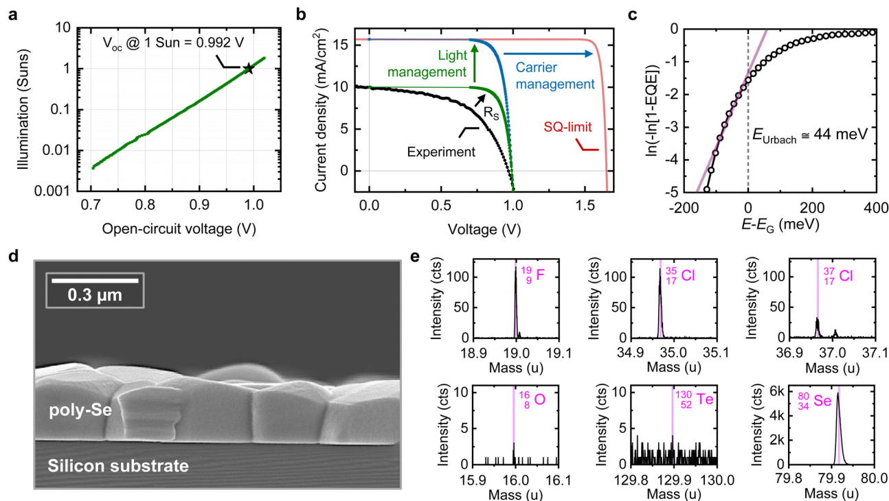
Fig. 7 Experimental device characterisation of a state-of-the-art selenium thin-film solar cell, and impurity analysis of the absorber. (a) Illumination-dependent open-circuit voltage ( \text{Suns-}V_{\text{oc}} ) demonstrating a record open-circuit voltage. 18 (b) Current–voltage ( JV ) curve of the experimental device, the reconstructed JV -curve from \text{Suns-}V_{\text{oc}} assuming the short-circuit current density from experiment (green) or the detailed-balance (DB) limit (blue), and the DB-limit JV curve – using the photovoltaic band gap of t-Se, E_{\text{g}}^{\text{PV}} , 27 obtained from the inflection point of the external quantum efficiency (EQE) spectrum. The photovoltaic losses which account for the difference between curves have been explicitly highlighted, including parasitic series resistance ( R_{\text{s}} ), light management (absorption losses), and carrier management (recombination losses, indirect band edges, etc.). (c) The Urbach band tailing derived from EQE measurements (Fig. S21, ESI†). (d) Cross-sectional scanning electron microscopy (SEM) of the thin-film selenium photo-absorber synthesised on a silicon substrate for impurity analysis. (e) Time-of-flight Secondary Ion Mass Spectrometry (ToF-SIMS) results, integrated while sputtering through the bulk of the selenium thin-film. Among the unintentional impurities, we detect F and Cl, whereas O and Te were only observed at the surface and interface with the substrate (see Section S7, ESI†).
