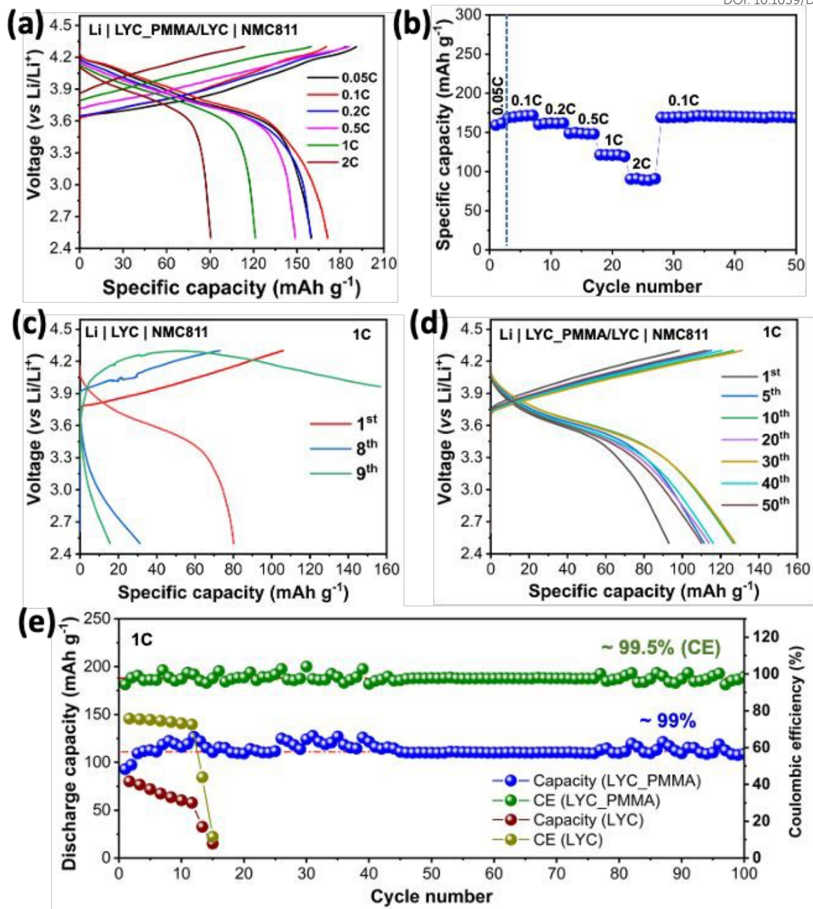
Fig. 4. a) Galvanostatic charge-discharge profiles and b) discharge capacity of Li|LYC_PMMA/LYC|NMC811 cells cycled at various rates as indicated (1C=200 mAh g -1 ). Galvanostatic charge-discharge profiles of c) Li|LYC|NMC811 and d) Li|LYC_PMMA/LYC|NMC811 cells cycled at the 1C rate, and e) discharge capacity and coulombic efficiency as functions of cycle number of the Li|LYC|NMC811 and Li|LYC_PMMA/LYC|NMC811 cells cycled at 1C.
