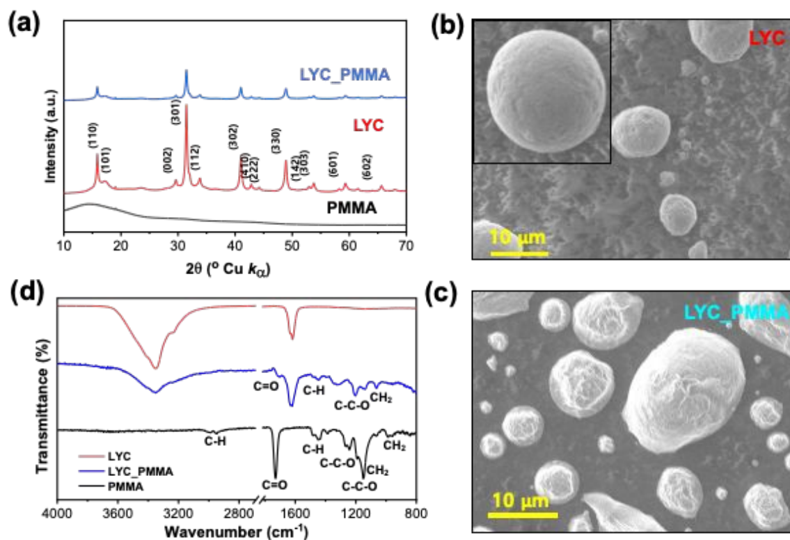
Fig. 1. a) XRD patterns of PMMA, LYC and LYC_PMMA. SEM images of LYC (b) and LYC_PMMA (c). d) FTIR spectra of PMMA, LYC and LYC_PMMA. The intensity of the LYC spectrum was reduced by 10 times for better comparison.
