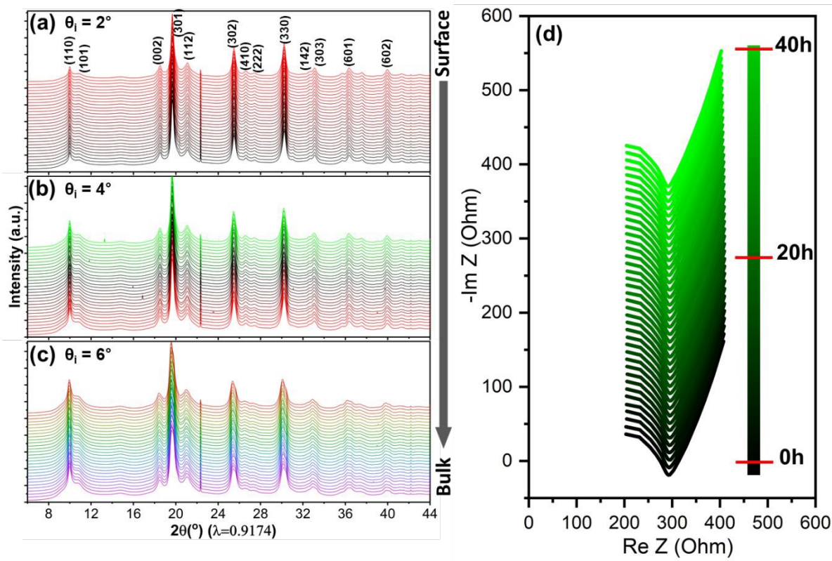
Fig. 6. Grazing-incidence XRD patterns of LYC_PMMA pellet as a function of air exposure time, collected at the incidence beam angle of a) 2^\circ , b) 4^\circ , and c) 6^\circ ( 2\theta ), respectively. The patterns were collected every 6 min within the total exposure time of 150 min. d) Operando time-resolved EIS spectra of a symmetric SS|LYC_PMMA|SS cell recorded as a function of air exposure time to evaluate the air stability of LYC_PMMA SE.
