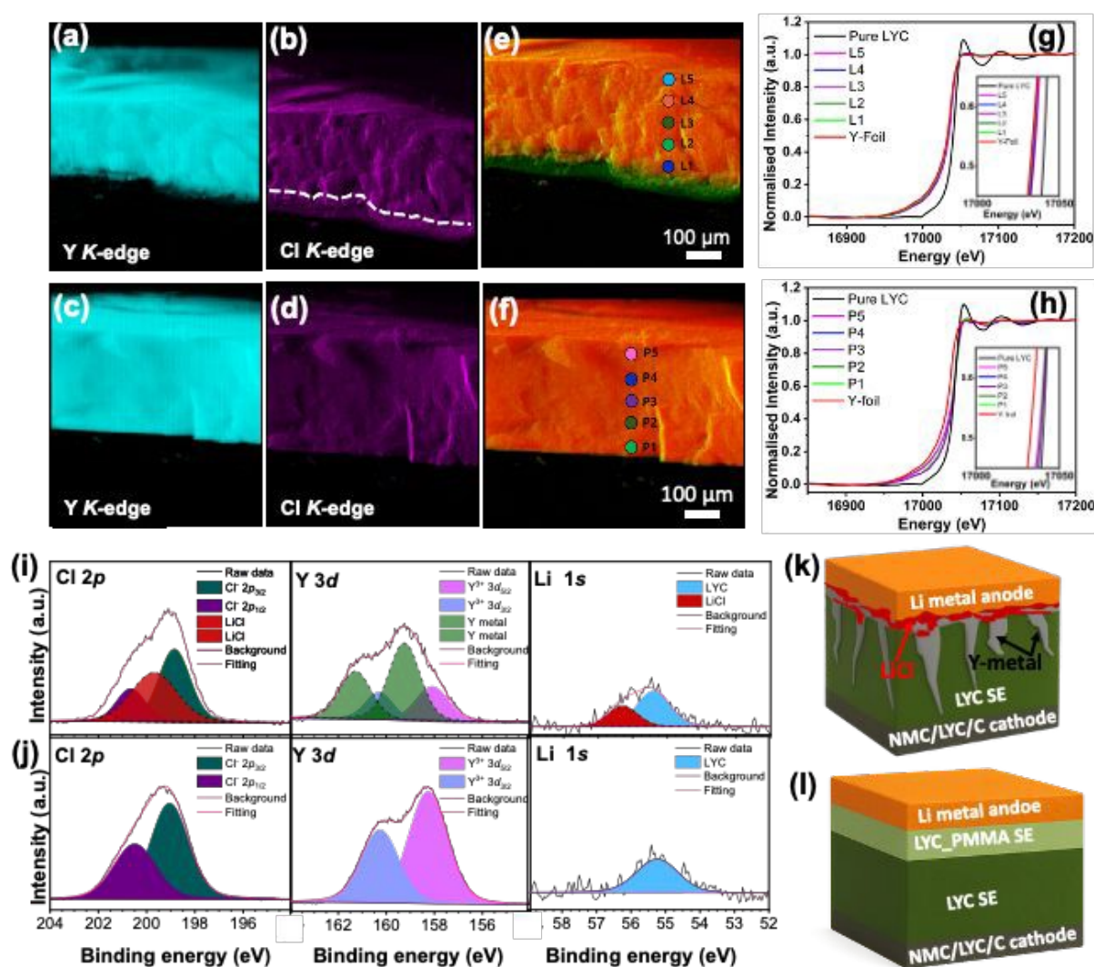
Fig. 5. \mu XRF maps of Y and Cl distribution on the electrolyte pellets recovered after continuous stripping/plating at a current density of 0.5 \text{ mA cm}^{-2} : a, b) Li|LYC|Li cell and c, d) Li|LYC_PMMA|Li cell. e, f) Combined \mu XRF maps of Y and Cl collected from the Li|LYC|Li and Li|LYC_PMMA|Li cells, respectively. (g, h) Y-K edge hard XAS spectra collected at various locations of the cycled LYC and LYC_PMMA pellets, respectively. The locations are labelled in e) and f). (i, j) XPS profiles of Y 3d , Cl 2p , and Li 1s collected on the cycled LYC and LYC_PMMA, respectively. (k, l) Schematics showing the evolution of the anode interface upon cycling of the Li|LYC|NMC811 and Li|LYC_PMMA/LYC|NMC811 cells, respectively.
