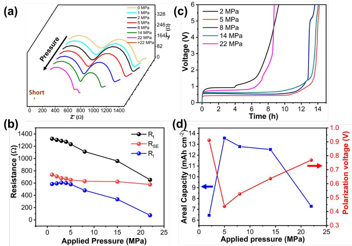
Fig. 2. a) EIS profiles and b) the relationships between various resistance components and the applied stack pressure of a Li|LYC_PMMA|Li cell, c) voltage profiles during unidirectional stripping of Li|LYC_PMMA|Li cells under various stack pressures, and d) areal capacity and polarization potential as functions of applied stack pressure.
