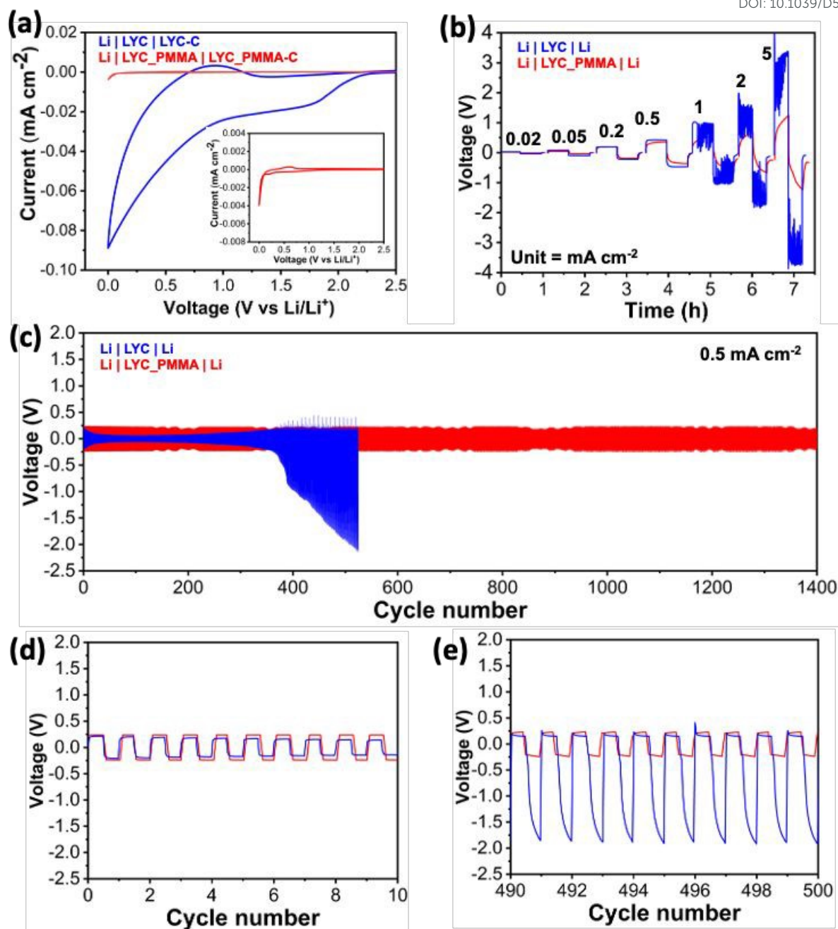
Fig. 3. a) Cyclic voltammograms of Li|LYC|LYC-C and Li|LYC_PMMA|LYC_PMMA-C cells at a scan rate of 0.1 \text{ mV s}^{-1} , b) Continuous stripping/plating of Li|LYC|Li and Li|LYC_PMMA|Li cells under various current densities ranging from 0.02 to 5 \text{ mA cm}^{-2} , and (c-e) long-term stripping/plating performance of the Li|LYC|Li and Li|LYC_PMMA|Li cells at a current density of 0.5 \text{ mA cm}^{-2} and a stacking pressure of 5 MPa. 1 full cycle is for 1 hour. (d-e) are the expanded views of the cycling profiles shown in the Fig. b. All measurements were carried out at room temperature.
