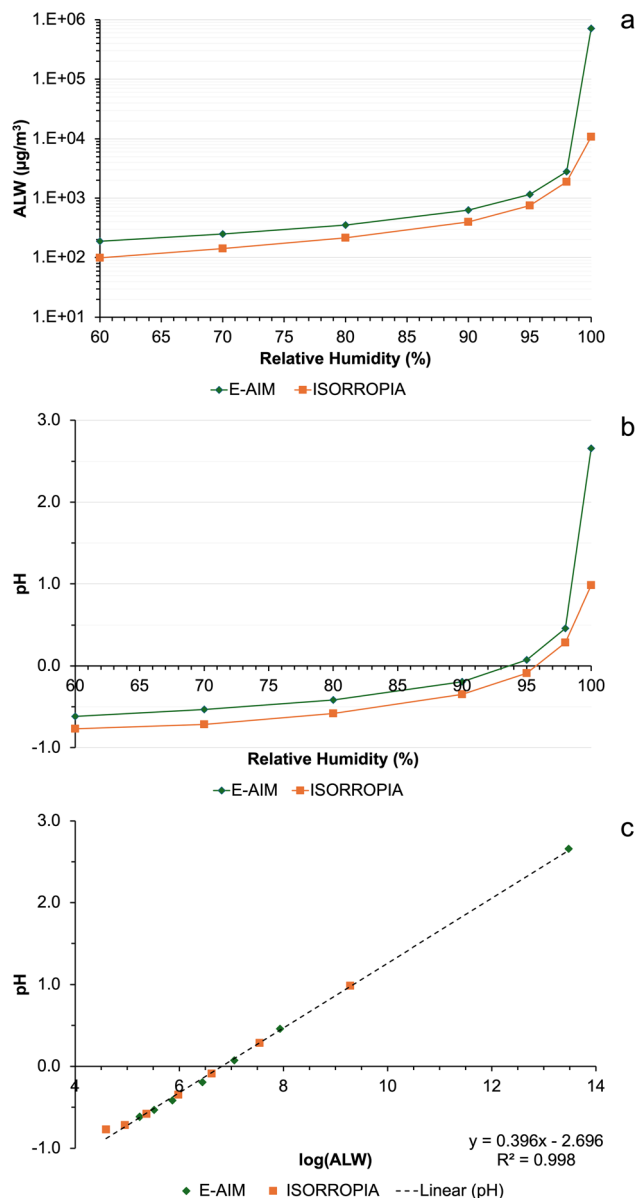
Fig. 2 Comparison of the outputs between E-AIM and ISORROPIA using the chemical composition of sample S1-0807-PM 0.5–0.25 (summit 1, 0.5–0.25 \mu\text{m} size fraction) as the input and varying relative humidity, between 60% and 100%: (a) aerosol liquid water (ALW) content, (b) pH, and (c) correlation between ALW and pH.
