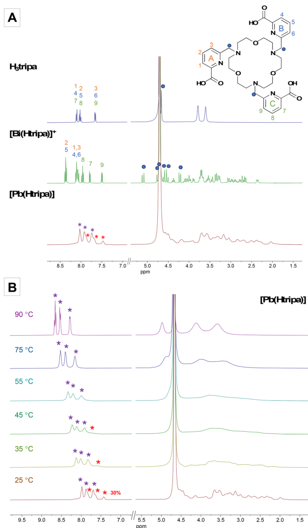
Fig. 2 (A) 1 H NMR spectra of H 3 tripa (400 MHz, D 2 O, pD 2), [Bi(Htripa)] + and [Pb(Htripa)] (400 MHz, D 2 O, pD 6–7). (B) Variable temperature 1 H NMR spectra of [Pb(Htripa)] (400 MHz, D 2 O, pD 7).
