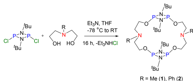
Scheme 1 Synthesis of macrocycles – [\{\text{P}(\mu\text{-N}^t\text{Bu})\}_2\{\text{O}(\text{CH}_2)_2\text{N}(\text{Me})(\text{CH}_2)_2\text{O}\}]_2 (1) and [\{\text{P}(\mu\text{-N}^t\text{Bu})\}_2\{\text{O}(\text{CH}_2)_2\text{N}(\text{Ph})(\text{CH}_2)_2\text{O}\}]_2 (2).
