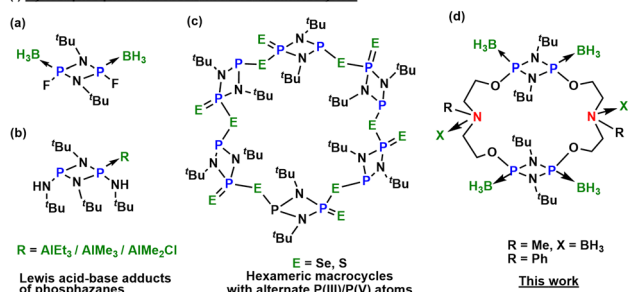
Fig. 1 (a and b) Selected examples of cyclodiphosphazane [\text{P}(\mu\text{-N}^t\text{Bu})]_2 -based adducts with main group Lewis acids; (c) an example of the heteroleptic \text{P}^{\text{V}}/\text{P}^{\text{III}} macrocycle; and (d) the newly synthesized first main group Lewis acid base adduct with phosphazane macrocycles.
