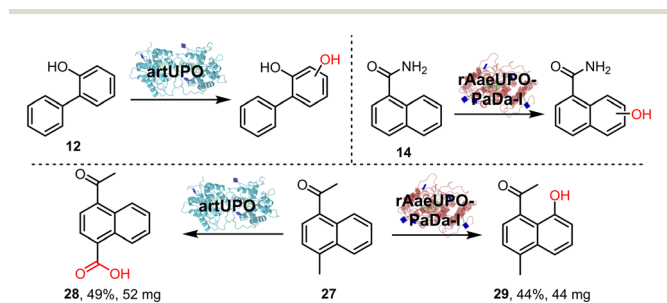
Scheme 2 UPO transformations of simple aromatics.
