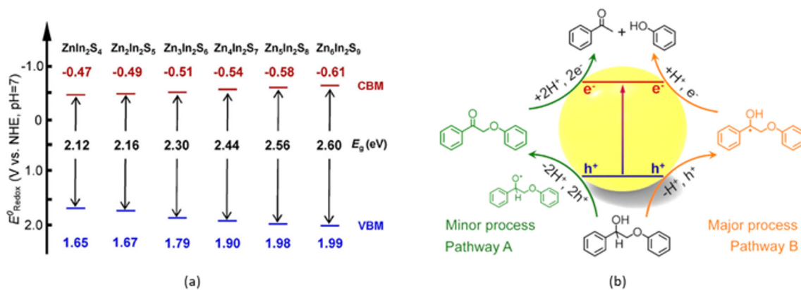
Scheme 4 (a) Band structure diagram of Zn m In 2 S m+3 ( m = 1-6 ); (b) proposed photocatalytic mechanism for \beta -O-4 bond cleavage in 2-phenoxy-1-phenylethanol over the Zn 4 In 2 S 7 catalyst (this scheme has been reproduced from ref. 16 with permission from Wiley-VCH, copyright 2019).
