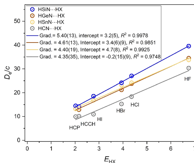
Fig. 8 Graphs of D_e/c versus E_{HX} for the four series HMN \cdots HX ( M = C, Si, Ge, Sn , ( X = F, Cl, Br, I, CCH, CP ) in which the atom M adjacent to that directly involved in the hydrogen bond belongs to Group 14.
