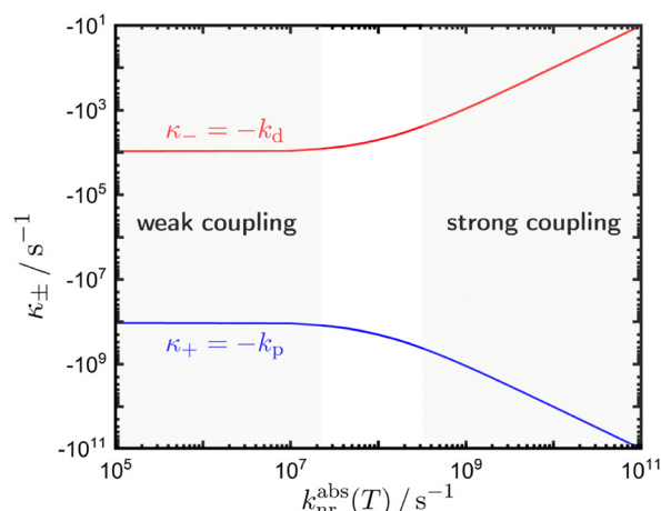
Fig. 4 Evolution of the two excited state rate constants k_{\pm} with the rate-determining constant k_{nr}^{abs}(T) that can be envisioned as a coupling strength between the two excited states |1\rangle and |2\rangle . Exemplary values were k_1 = 10 \text{ ms}^{-1} and K_2 = 0.1 \text{ ns}^{-1} (for definitions see text) representative for a TADF emitter. Most practical TADF emitters tend to be in the weak coupling regime. Inorganic emitters such as the lanthanoid ions or \text{Cr}^{3+} are much more commonly in the strong coupling regime at ambient temperatures, which is relevant to ratiometric thermometry with steady-state spectra.
