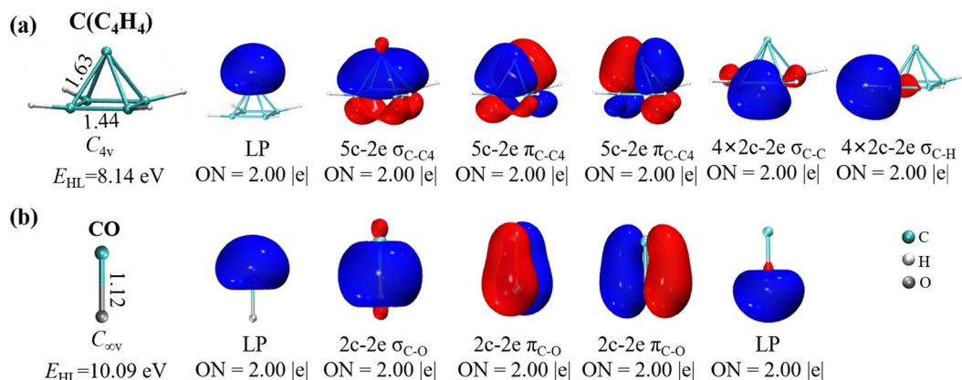
Fig. 1 PBE0/def2-TZVP optimized structures with key bond lengths, AdNDP localized bonds, and electronic occupation numbers (ONs) of the (a) \text{C}(\text{C}_4\text{H}_4) and (b) CO molecules. The carbon, hydrogen and oxygen atoms are represented by cyan, white and grey balls, respectively.
