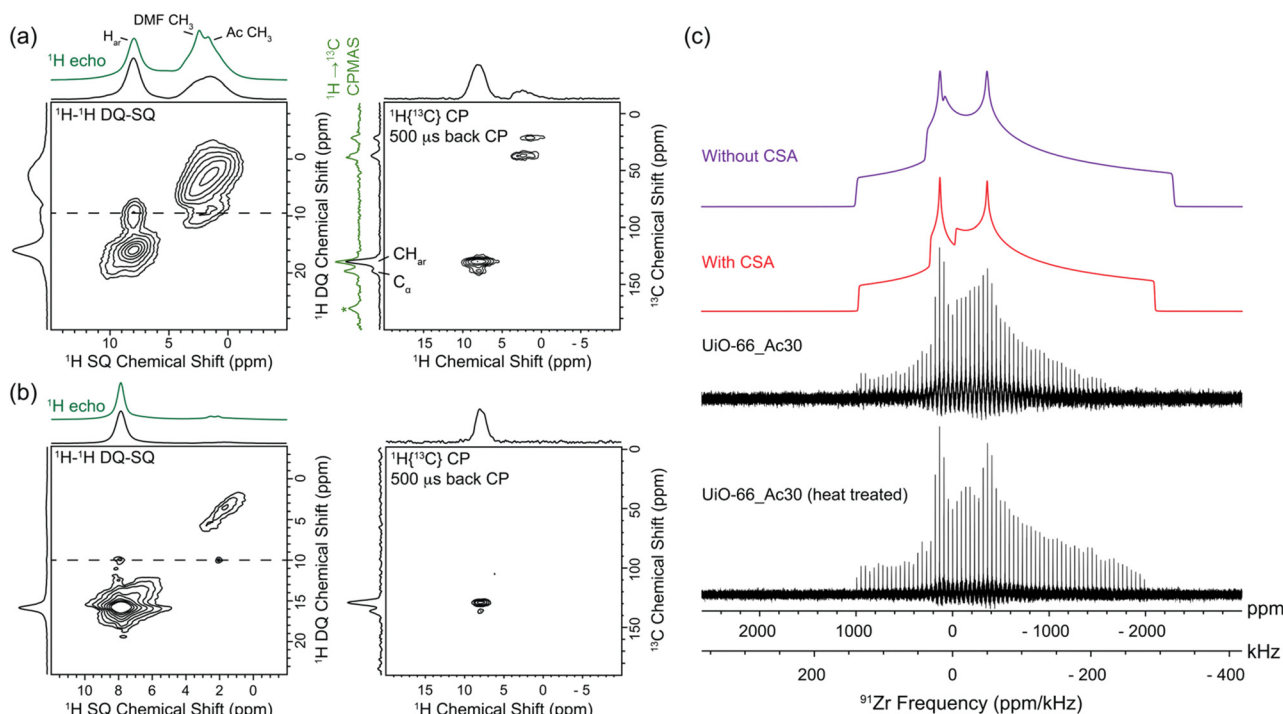
Fig. 2 (a) and (b) Fast MAS 2D ^1\text{H} SQ-DQ (left) and 2D ^1\text{H} ( ^{13}\text{C} ) cross polarization heteronuclear correlation (right) NMR spectra of UiO-66 synthesized with acetic acid modulator (denoted UiO-66_Ac30) and the same sample of UiO-66 treated at 300 °C (labelled UiO-66_Ac30 (heat-treated)). The corresponding 1D ^1\text{H} spin echo spectra are also shown (green traces). Spectra were acquired at a MAS frequency of 50 kHz and a magnetic field of 9.4 T. (c) Static and simulated static 35.2 T ^{91}\text{Zr} NMR spectra of UiO-66_Ac30 and UiO-66_Ac30 (heat-treated). Analytical simulations of the ^{91}\text{Zr} second-order quadrupole patterns are shown with CSA ( \delta_{\text{iso}} = -100 ppm, \Omega = 200 ppm, \kappa = 0.0 , C_Q = 32.5 MHz, \eta = 0.79 , \alpha = 0 , \beta = 0 , \gamma = 0 ) and without CSA ( \delta_{\text{iso}} = -100 ppm, C_Q = 34.5 MHz, \eta = 0.79 ), where \Omega and \kappa are the span and skew of the CSA tensor and \alpha , \beta , and \gamma are the Euler angles between the EFG and CS tensors.
