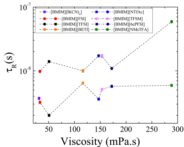
Fig. 5 Average rotational time of [BMIM] + (squared symbols) and the corresponding anions (circular symbols) that contain ^{19}\text{F} in their chemical structures ([FSAI] − , [BETI] − , [NTfAc] − , [TFSM] − , [6cPFSI] − and [NMsTFA] − ) as a function of viscosity, at 25 °C. Viscosity values were taken with permission from ref. 16. Rotational times of [BMIM] + and [TFSI] − in [BMIM][TFSI] are included for comparison purposes and are taken with permission from ref. 20. The dashed lines are guides to the eye.
