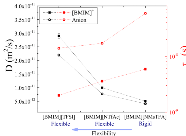
Fig. 6 Diffusion coefficients (black symbols) and rotational times (red symbols) of [BMIM] + (squared solid symbols) and the corresponding anion (circular hollow symbols) in the three ILs of group A, at 25 °C. Rotational times of [BMIM] + and [TFSI] - in [BMIM][TFSI] are taken with permission from ref. 20. Dashed lines are guides to the eye.
