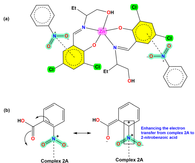
Scheme 5 (a) Schematic representation of electron transfer from complex 2A to 2-nitrobenzoic acid; (b) schematic representation of the canonical structures of 2-nitrobenzoic acid and its impact on the quenching mechanism.
