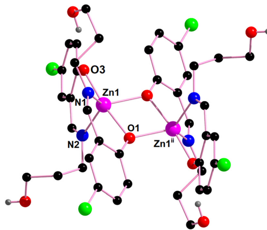
Fig. 9 Perspective view of complex 4 with selective atom numbering. Symmetry transformation \text{ii} = 1 - x, 1 - y, 1 - z .
