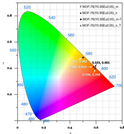
Fig. 13 Chromaticity (CIE) diagram comparing the color coordinates of synthesized MOF-76(Y 0.95 Eu 0.05 ) n and MOF-76(Y 0.95 Eu 0.05 ) m compounds, and the corresponding ones to the MOF-76(Y 0.95 Eu 0.05 ) m-T and MOF-76(Y 0.95 Eu 0.05 ) n-T phases. The purity color is summarized below the graph. The CIE image was made using the Sci-Sim website. 70
