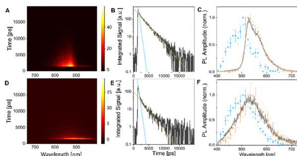
Fig. 3 Streak camera data of HA(OMe)-T in CHCl 3 (A)–(C) and CHCl 3 /MeOH (20:80) (D)–(F). (A) and (D) Streak camera measurements (0.1 \mu g mL -1 ). (B) and (E) Time traces integrated over the whole spectral range of the streak camera data. The straight lines indicate the decays with a short (cyan) and long lifetime (orange). (C) and (F) Decay associated spectra (DAS) obtained from a global fit of the Streak data, as well as the integrated spectrum of the streak camera (grey).
